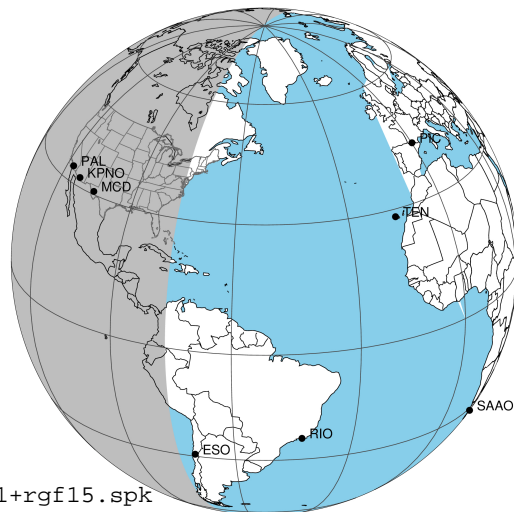
2025-09-22T10:55:40.4900 α: 07 30 43.7885 δ: +21 48 33.2393 C/A ***** PA 188.08 deg v_sky +23.28 km/s D 05.46 AU Credit: Styled after SORA/Lucky Star
