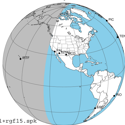
2025-09-27T14:14:59.0700 α: 07 33 41.8447 δ: +21 42 30.807 C/A ***** PA 188.27 deg v_sky +21.13 km/s D 05.39 AU Credit: Styled after SORA/Lucky Star
