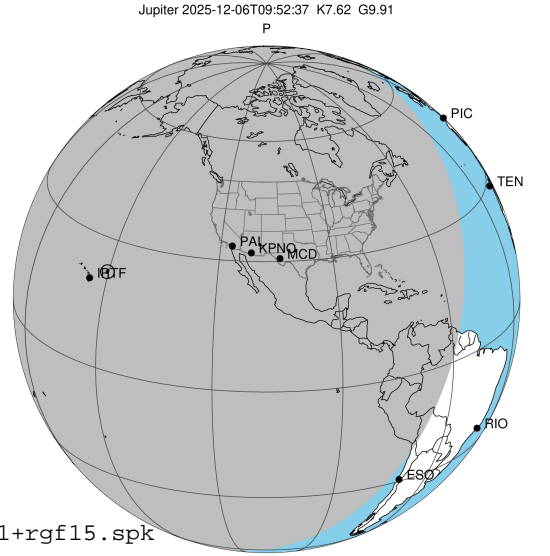
2025-12-06T09:52:37.3300 au: 07 42 45.0745 s: +21 31 13.6989 C/A ***** PA 191.82 deg v_sky -10.56 km/s D 04.41 AU Credit: Styled after SORA/Lucky Star
