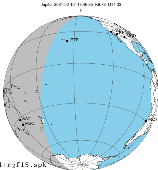
2031-02-10T17:46:35.0400 @: 17 28 47.13041 & -22 41 47.707 C/A ***** PA 183.17 deg v_sky +28.69 km/s D 05.77 AU Credit: Styled after SORA/Lucky Star
