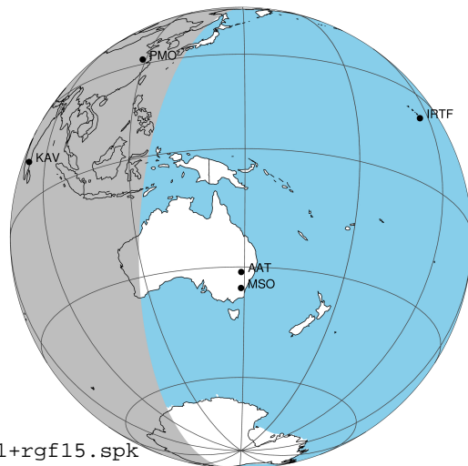
2031-02-16T21:52:10.2400 ex: 17 33 02.0153 s: -22 45 06.917 C/A 0.566" PA 182.72 deg v_sky +26.30 km/s D 05.68 AU Credit: Styled after SORA/Lucky Star
