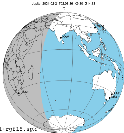
2031-02-21T02:08:36.9300 α: 17 35 43.9118 δ: -22 47 06.546 C/A ***** PA 2.47 deg v_sky +24.60 km/s D 05.62 AU Credit: Styled after SORA/Lucky Star
