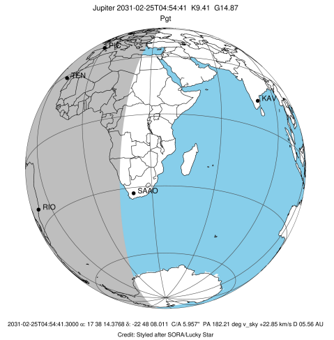
Jupiter 2031-02-25T04:54:41 K9.41 G14.87
