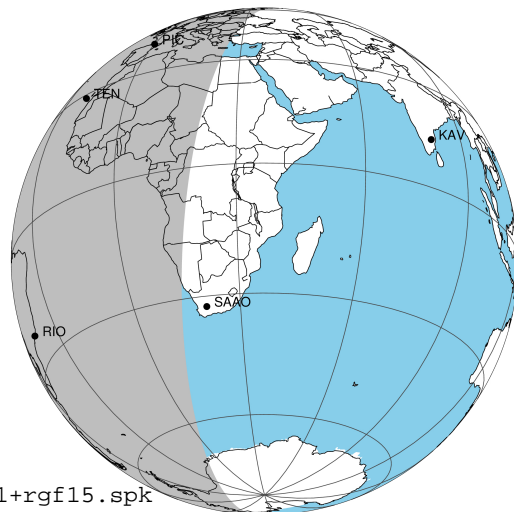
2031-02-25T04:54:41.3000 cc: 17 38 14.3768 s: -22 48 08.011 C/A 5.957" PA 182.21 deg v_sky +22.85 km/s D 05.56 AU Credit: Styled after SORA/Lucky Star
