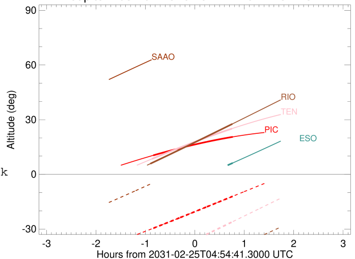
Jupiter 2031-02-25T04:54:41 K9.41 G14.87
