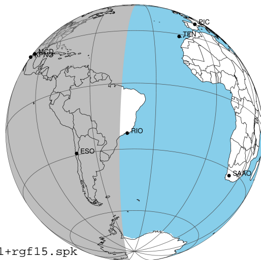
2031-03-11T09:11:09.9200 a: 17 45 36.1935 s: -22 51 10.608 C/A ***** PA 181.45 deg v_sky +16.52 km/s D 05.33 AU Credit: Styled after SORA/Lucky Star
