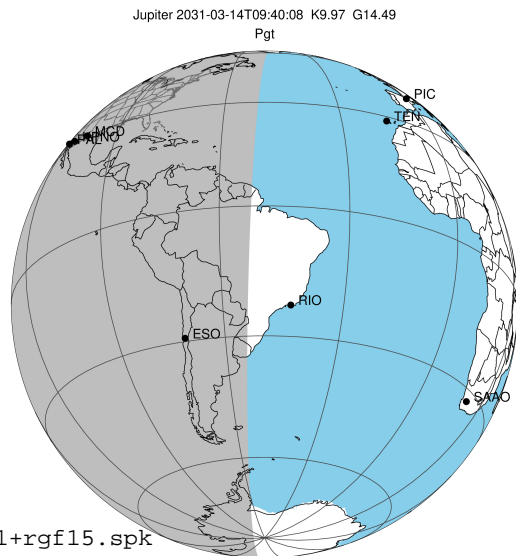
2031-03-14T09:40:08.0300 a: 17 46 53.76986 s: -22 51 37.304 C/A ***** PA 181.32 deg v_sky +15.13 km/s D 05.28 AU Credit: Styled after SORA/Lucky Star
