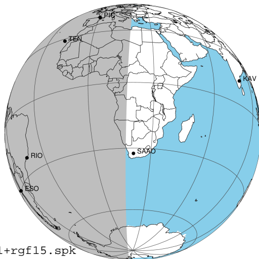
2031-03-15T04:56:39.2800 az: 17 47 13.3488 δ: -22 51 50.680 C/A ***** PA 181.29 deg v_sky +14.75 km/s D 05.27 AU Credit: Styled after SORA/Lucky Star
