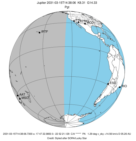
Jupiter 2031-03-15T14:38:06 K8.31 G14.33
