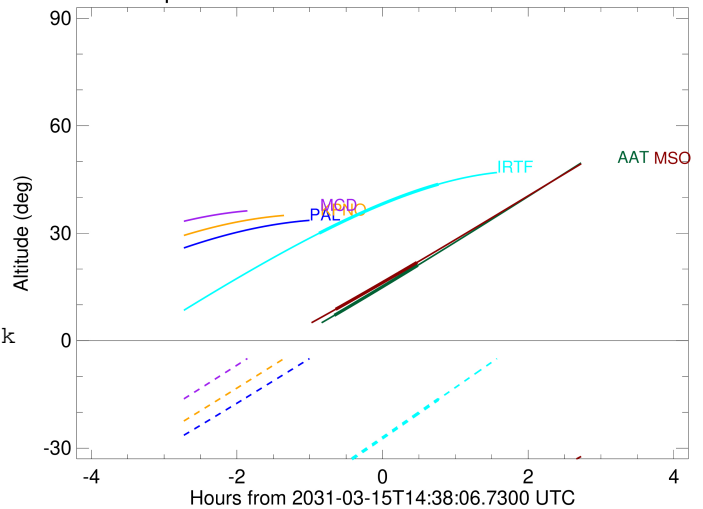
Jupiter 2031-03-15T14:38:06 K8.31 G14.33
