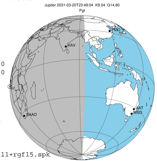
2031-03-20T23:49:04.5500 α: 17 49 21.0451 δ: -22 52 56.519 C/A ***** PA 1.12 deg v_sky +12.01 km/s D 05.18 AU Credit: Styled after SORA/Lucky Star
