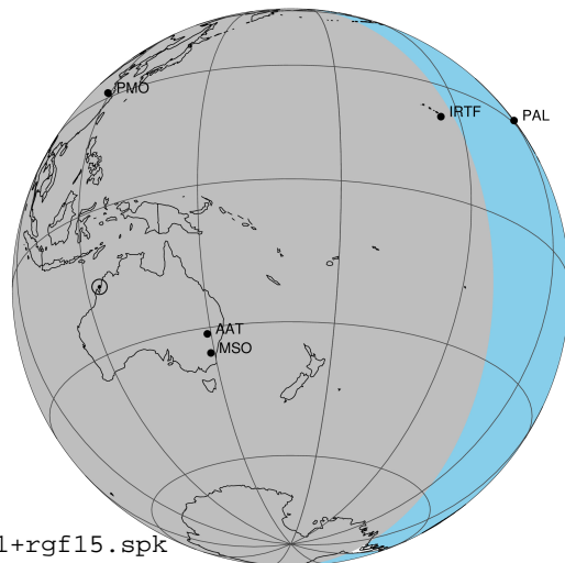
2031-05-05T15:41:06.1100 α: 17 50 55.67289 δ: -22 53 28.087 C/A ***** PA 180.23 deg v_sky - 8.38 km/s D 04.52 AU Credit: Styled after SORA/Lucky Star
