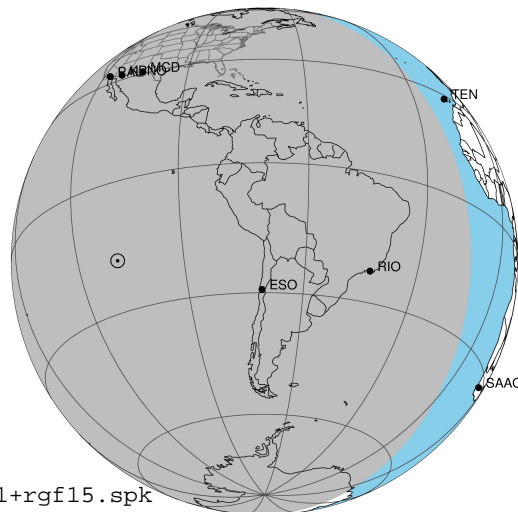
2031-05-13T07:07:13.2500 a: 17 48 32.7597 δ: -22 53 15.682 C/A ***** PA 180.47 deg v_sky -10.97 km/s D 04.44 AU Credit: Styled after SORA/Lucky Star
