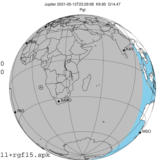
2031-05-13T23:29:58.2400 α: 17 48 18.0383 δ: -22 53 48.826 C/A ***** PA 0.48 deg v_sky -11.18 km/s D 04.43 AU Credit: Styled after SORA/Lucky Star
