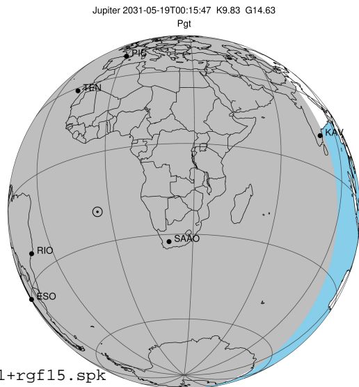
2031-05-19T00:15:47.6600 α: 17 46 20.5873 δ: -22 53 37.388 C/A ***** PA 0.65 deg v_sky -12.65 km/s D 04.39 AU Credit: Styled after SORA/Lucky Star
