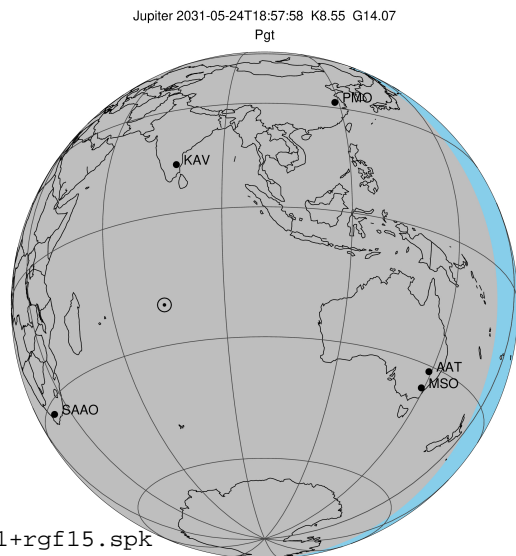
2031-05-24T18:57:58.6900 a: 17 43 47.8608 s: -22 52 59.372 C/A 6.325" PA 0.87 deg v_sky -14.05 km/s D 04.34 AU Credit: Styled after SORA/Lucky Star
