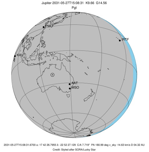
Jupiter 2031-05-27T15:08:31 K9.66 G14.56
