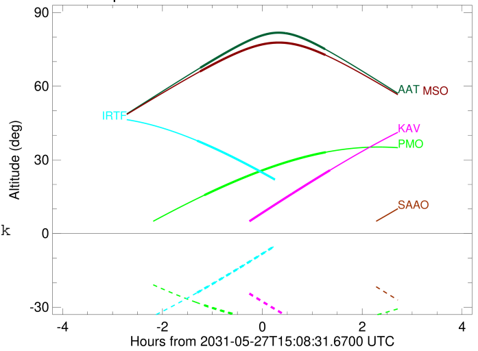
Jupiter 2031-05-27T15:08:31 K9.66 G14.56
