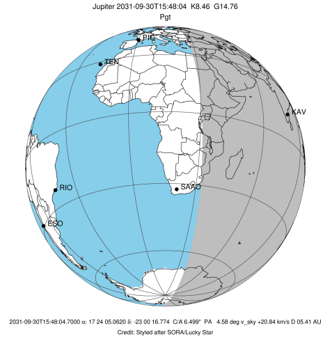
Jupiter 2031-09-30T15:48:04 K8.46 G14.76
