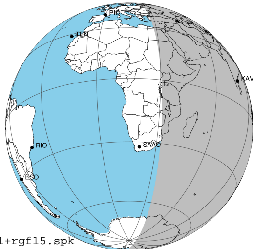
2031-09-30T15:48:04.7000 α: 17 24 05.0620 δ: -23 00 16.774 C/A 6.499° PA 4.58 deg v_sky +20.84 km/s D 05.41 AU Credit: Styled after SORA/Lucky Star
