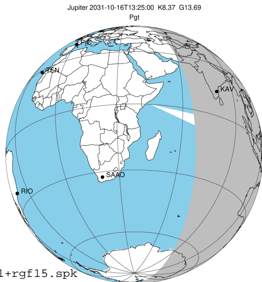
2031-10-16T13:25:00.7500 cc: 17 34 03.1204 s: -23 09 35.682 C/A 1.073° PA 183.31 deg v_sky +27.37 km/s D 05.64 AU Credit: Styled after SORA/Lucky Star
