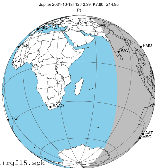
2031-10-18T12:42:39.4600 α: 17 35 26.4779 β: -23 10 59.759 C/A ***** PA 3.14 deg v_sky +28.13 km/s D 05.67 AU Credit: Styled after SORA/Lucky Star
