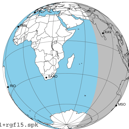
2031-10-18T12:58:56.4500 α: 17 35 26.9744 δ: -23 10 57.062 C/A ***** PA 3.14 deg v_sky +28.13 km/s D 05.67 AU Credit: Styled after SORA/Lucky Star
