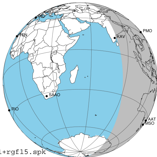
2031-10-22T12:10:34.6000 cc: 17 38 20.6488 s: -23 12 42.339 C/A 4.2677 PA 182.82 deg v_sky +29.60 km/s D 05.72 AU Credit: Styled after SORA/Lucky Star
