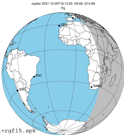
2031-10-26T16:13:20.7100 a: 17 41 30.7142 s: -23 14 55.998 C/A 8.628" PA 2.46 deg v_sky +31.07 km/s D 05.77 AU Credit: Styled after SORA/Lucky Star
