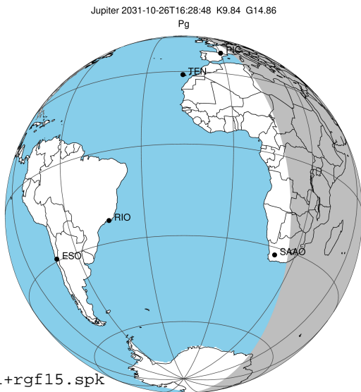
2031-10-26T16:28:48.6800 α: 17 41 31.2305 δ: -23 14 50.922 C/A 3.251" PA 2.47 deg v_sky +31.07 km/s D 05.77 AU Credit: Styled after SORA/Lucky Star
