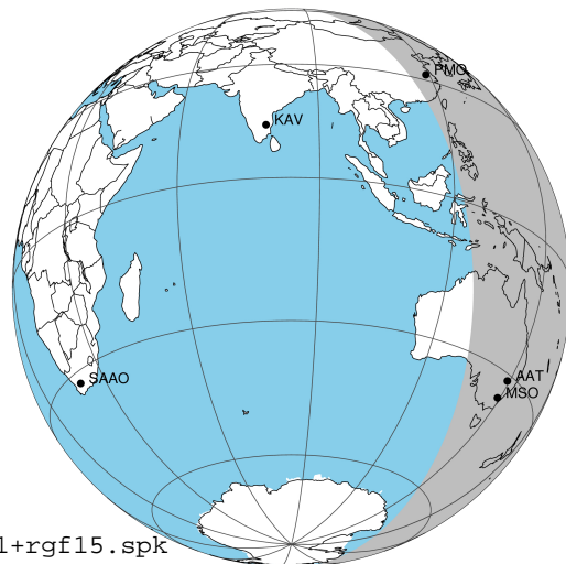
2031-10-31T09:32:28.2500 a: 17 45 14.9269 s: -23 16 39.099 C/A ***** PA 182.06 deg v_sky +32.64 km/s D 05.83 AU Credit: Styled after SORA/Lucky Star
