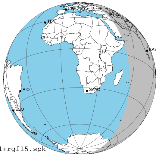
2031-10-31T14:11:10.7800 α: 17 45 24.2675 δ: -23 16 58.501 C/A 4.698" PA 2.04 deg v_sky +32.71 km/s D 05.83 AU Credit: Styled after SORA/Lucky Star
