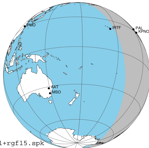
2031-11-01T03:24:52.8100 a: 17 45 51.11256 s: -23 16 49.23445 C/A ***** PA 181.99 deg v_sky +32.89 km/s D 05.83 AU Credit: Styled after SORA/Lucky Star
