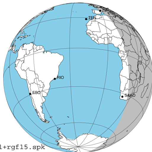
2031-11-02T16:35:26.4800 ex: 17 47 06.9847 s: -23 17 40.298 C/A 1.538" PA 181.86 deg v_sky +33.38 km/s D 05.85 AU Credit: Styled after SORA/Lucky Star
