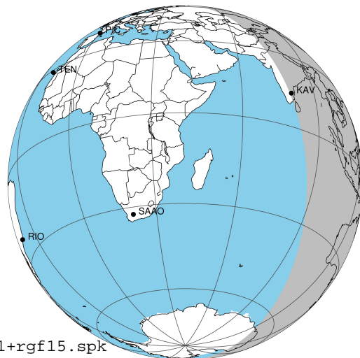
2031-11-03T12:15:03.8300 α: 17 47 47.4597 δ: -23 18 15.998 C/A ***** PA 1.77 deg v_sky +33.64 km/s D 05.86 AU Credit: Styled after SORA/Lucky Star
