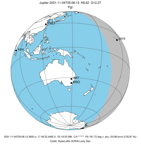
Jupiter 2031-11-04T05:06:13 K8.62 G12.27
