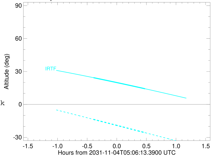
Jupiter 2031-11-04T05:06:13 K8.62 G12.27
