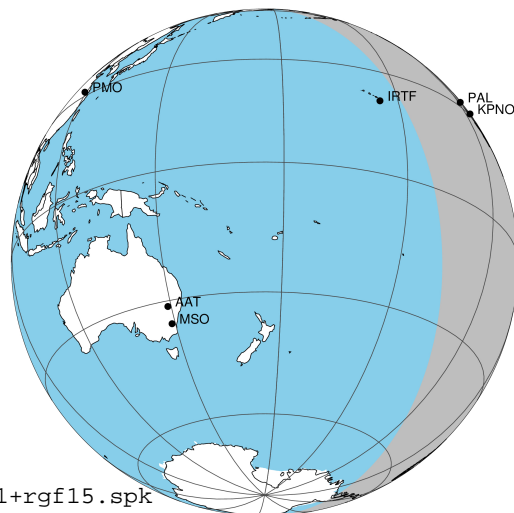
2031-11-05T03:11:58.6700 a: 17 49 08.5309 s: -23 18 16.825 C/A ***** PA 181.64 deg v_sky +34.14 km/s D 05.88 AU Credit: Styled after SORA/Lucky Star
