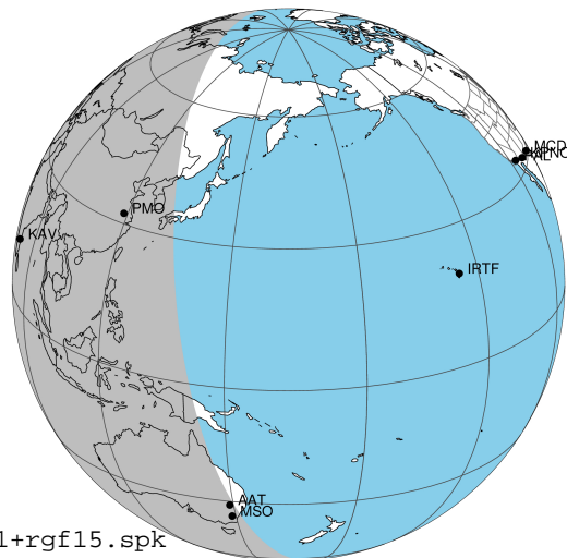
2036-08-19T20:34:49.9900 α: 05 21 37.5487 δ: +22 32 23.143 C/A ***** PA 176.18 deg v_sky +24.87 km/s D 05.39 AU Credit: Styled after SORA/Lucky Star
