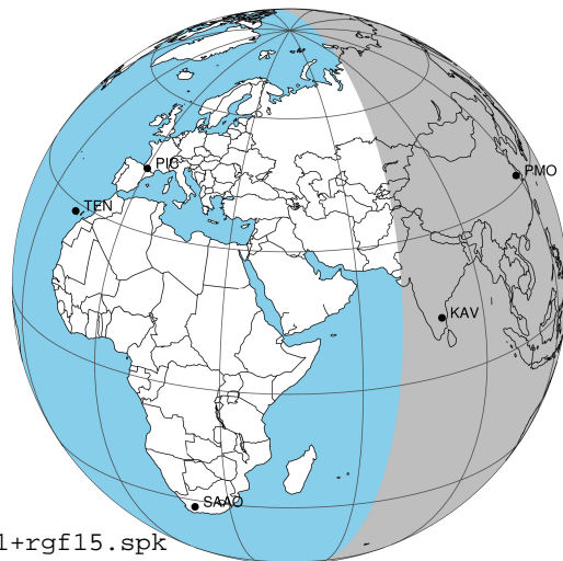
2037-04-03T13:31:05.0800 α: 05 16 28.3734 δ: +22 50 23.488 C/A ***** PA 354.78 deg v_sky +24.60 km/s D 05.45 AU Credit: Styled after SORA/Lucky Star
