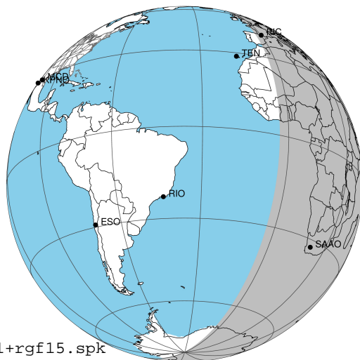
2042-09-20T18:06:13.1900 α: 15 39 50.0782 δ: -18 50 52.356 C/A 1.466° PA 14.27 deg v_sky +27.80 km/s D 05.79 AU Credit: Styled after SORA/Lucky Star
