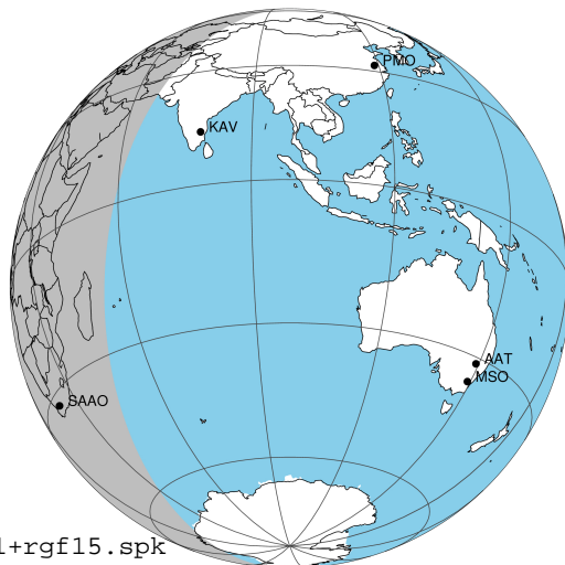
2043-02-03T02:16:52.3900 @: 17 38 38.9807 & -22 52 55.031 C/A 3.552" PA 2.30 deg v_sky +32.98 km/s D 05.91 AU Credit: Styled after SORA/Lucky Star
