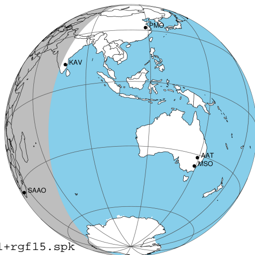
2043-02-04T01:21:45.3200 α: 17 39 24.9593 δ: -22 53 32.868 C/A ***** PA 2.22 deg v_sky +32.66 km/s D 05.90 AU Credit: Styled after SORA/Lucky Star
