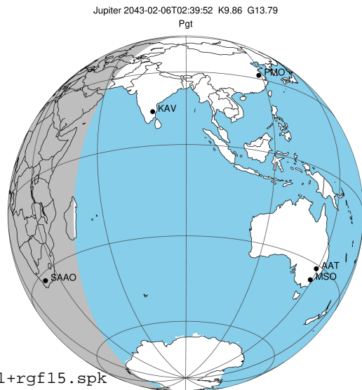
2043-02-06T02:39:52.7500 @: 17 41 02.1152 & -22 54 10.883 C/A 4.227" PA 2.06 deg v_sky +31.98 km/s D 05.88 AU Credit: Styled after SORA/Lucky Star
