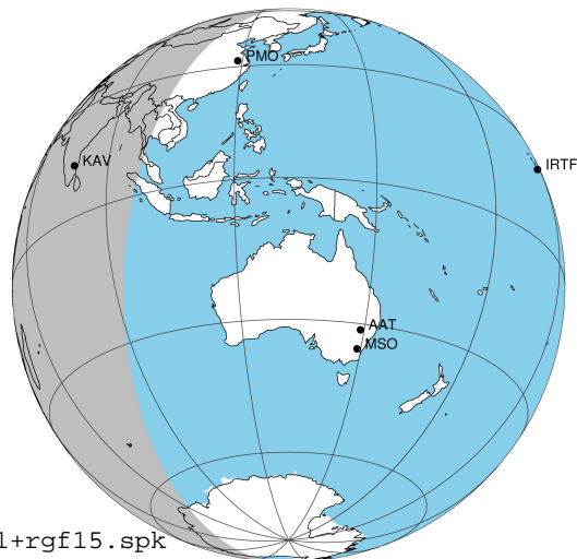
2043-02-08T23:44:27.5300 a: 17 43 15.4611 s: -22 54 52.730 C/A ***** PA 181.83 deg v_sky +30.99 km/s D 05.84 AU Credit: Styled after SORA/Lucky Star
