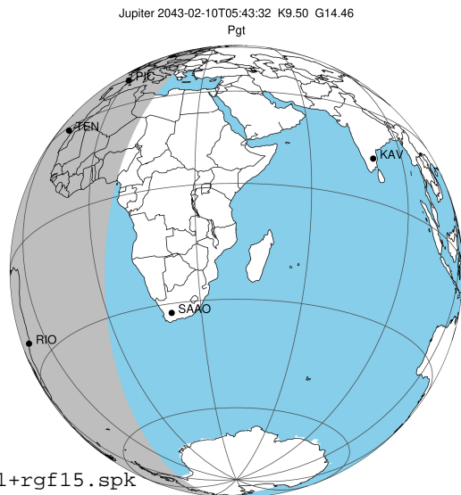
2043-02-10T05:43:32.7600 @: 17 44 12.2541 s -22 55 23.329 C/A ***** PA 181.73 deg v_sky +30.54 km/s D 05.82 AU Credit: Styled after SORA/Lucky Star
