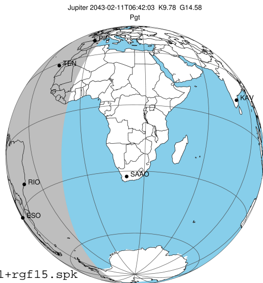
2043-02-11T06:42:03.3300 a: 17 44 59.0778 s: -22 55 36.240 C/A ***** PA 181.65 deg v_sky +30.17 km/s D 05.81 AU Credit: Styled after SORA/Lucky Star
