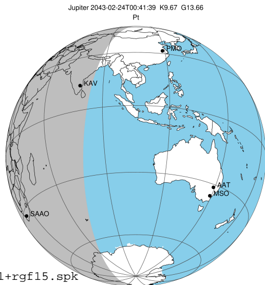
2043-02-24T00:41:39.6700 α: 17 53 52.1804 δ: -22 58 47.102 C/A ***** PA 0.78 deg v_sky +25.25 km/s D 05.63 AU Credit: Styled after SORA/Lucky Star
