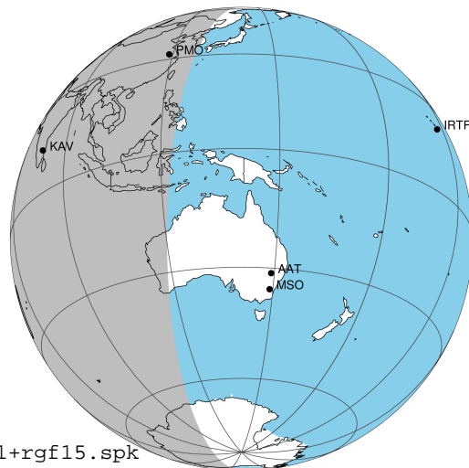
2043-03-01T21:59:55.7100 a: 17 57 30.7338 & -22 59 00.540 C/A 0.119" PA 0.39 deg v_sky +22.80 km/s D 05.54 AU Credit: Styled after SORA/Lucky Star
