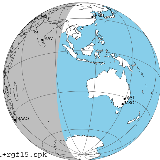
2043-03-02T00:02:52.3400 a: 17 57 33.7726 s: -22 58 42.170 C/A ***** PA 180.41 deg v_sky +22.76 km/s D 05.54 AU Credit: Styled after SORA/Lucky Star
