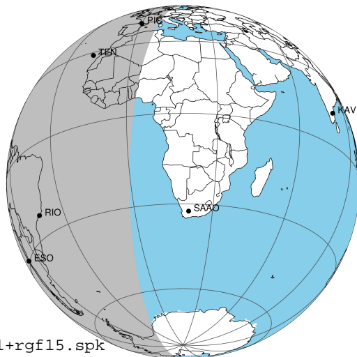
2043-03-03T06:02:22:5400 a: 17 58 17.6312 s & -22 58 53.030 C/A ***** PA 180.34 deg v_sky +22.23 km/s D 05.52 AU Credit: Styled after SORA/Lucky Star
