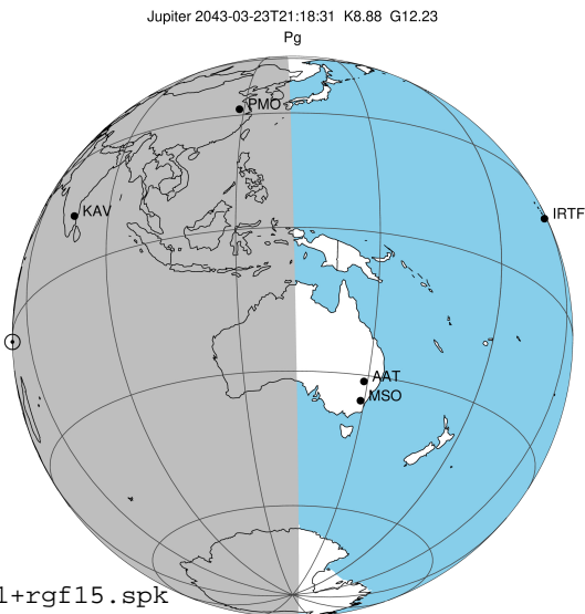
2043-03-23T21:18:31.5200 a: 18 08 00.8539 s: -22 58 31.252 C/A ***** PA 179.48 deg v_sky +12.82 km/s D 05.19 AU Credit: Styled after SORA/Lucky Star
