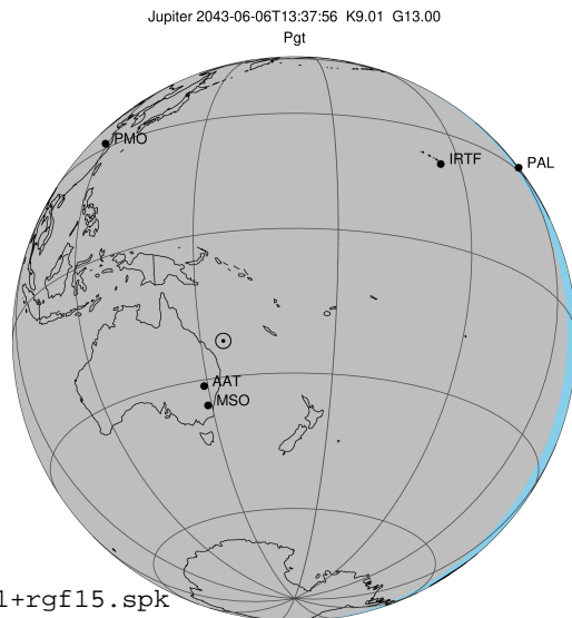
2043-06-06T13:37:56.1300 at: 17 59 05.9808 s: -23 03 55.125 C/A 6.010° PA 359.21 deg v_sky -15.46 km/s D 04.28 AU Credit: Styled after SORA/Lucky Star
