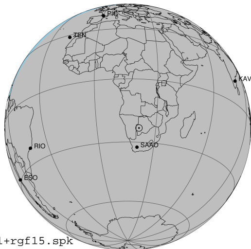
2043-06-24T22:36:45.4200 a: 17 49 03.7915 s: -23 04 23.859 C/A ***** PA 180.04 deg v_sky -16.30 km/s D 04.25 AU Credit: Styled after SORA/Lucky Star
