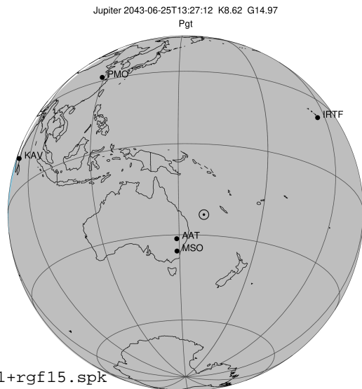
2043-06-25T13:27:12.9200 a: 17 48 43.3506 s: -23 04 25.501 C/A ***** PA 180.06 deg v_sky -16.27 km/s D 04.25 AU Credit: Styled after SORA/Lucky Star
