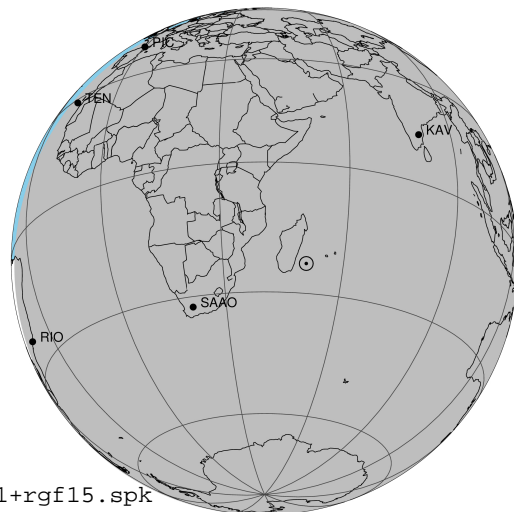
2043-06-28T20:40:50.7400 a: 17 46 55.1188 s -23 04 15.365 C/A ***** PA 180.19 deg v_sky -16.04 km/s D 0.26 AU Credit: Styled after SORA/Lucky Star
